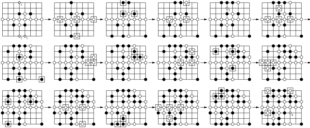
FIGURE 16. Under the hypothesis that one of the diamonds marked 1 has color \circ and the other has color \bullet and that the diamond marked 2 has color \bullet , the diamond marked 3 must have color \circ (stacked rows). The diamond marked 4 cannot be colored.
