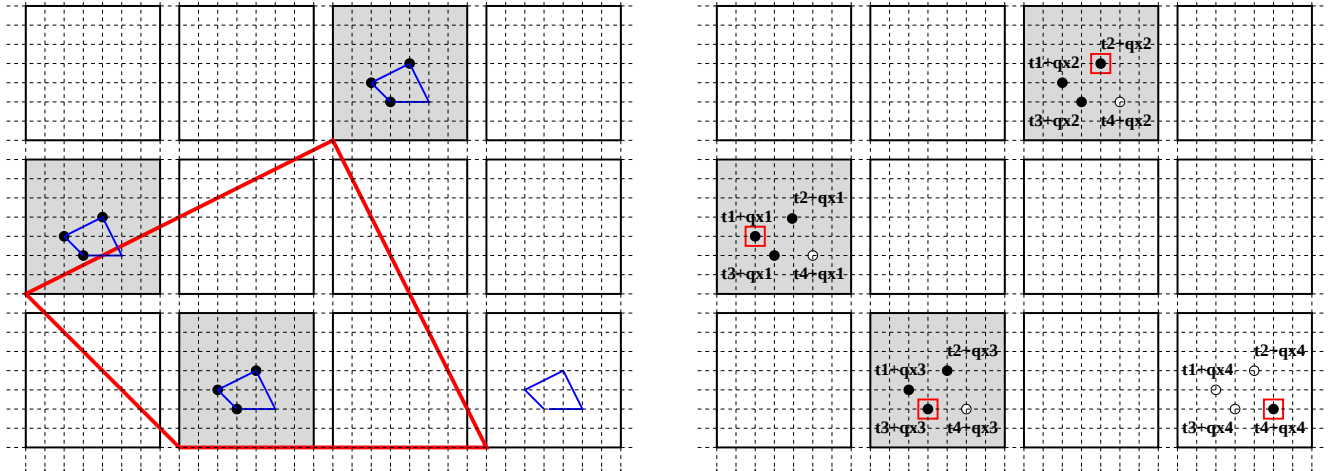
FIGURE 4. An example of the configuration from Lemma 3 is describing. In this example, the points \mathbf{t}_j + q\mathbf{x}_i are elements of shaded subgrids A_{\mathbf{x}_i} .
