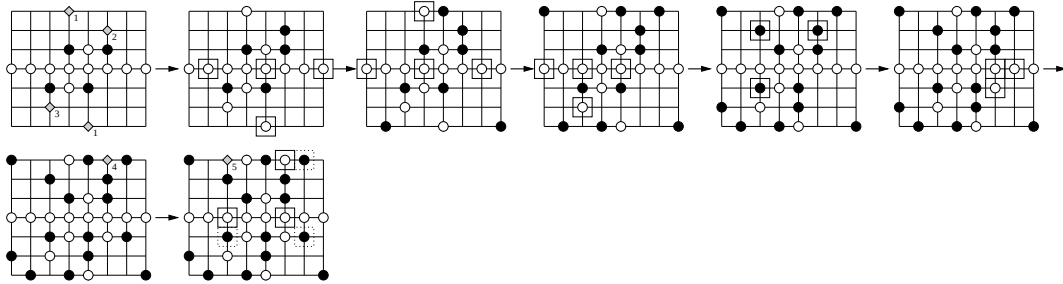
FIGURE 12. Under the hypothesis that the diamonds marked 1 have color \circ , the diamond marked 2 has color \bullet , and the diamond marked 3 has color \circ , the diamond marked 4 must have color \circ (staggered rows). The diamond marked 5 cannot be colored.
