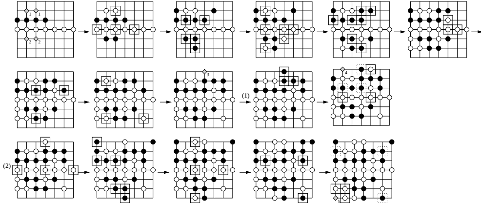
FIGURE 6. Both diamonds marked 1 must have color \circ , while both diamonds marked 2 must have color \bullet , else we have a monochromatic square. (1) examines the case where the diamond marked 3 has color \bullet ; here, the diamond marked 4 cannot be colored. (2) examines the case where the diamond marked 3 has color \circ ; here, the diamond marked 5 cannot be colored.
