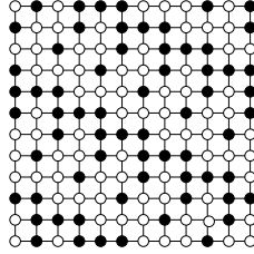
FIGURE 1. A 2-coloring of [12]^2 with no monochromatic square.
