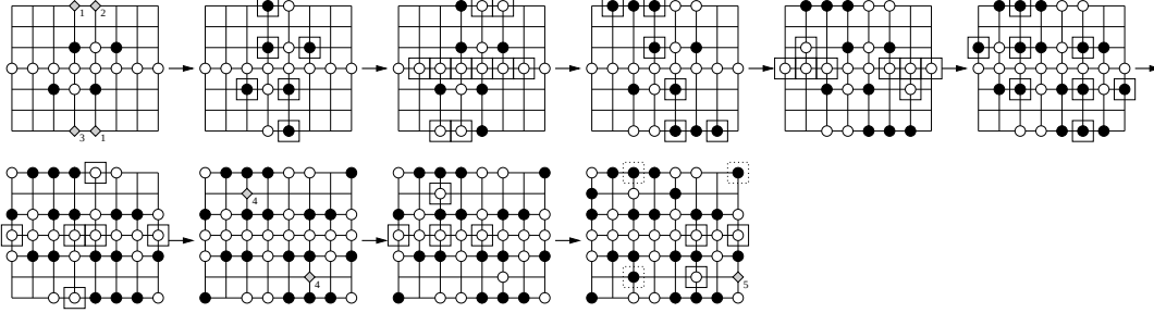
FIGURE 15. Under the hypothesis that both diamonds marked 1 have color \bullet and both diamonds marked 2 and 3 have color \circ , the diamonds marked 4 must have color \circ (stacked rows). This shows that the diamond marked 5 cannot be colored.
