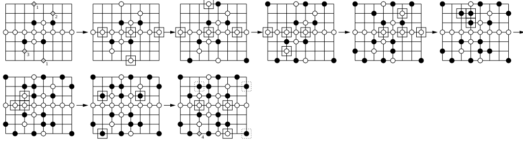
FIGURE 10. Under the hypothesis that the diamonds marked 1, 2, and 3 all have color \circ , the diamond marked 4 cannot be colored.
