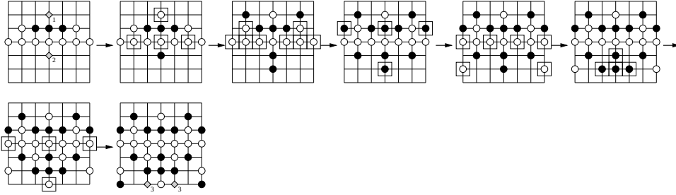
FIGURE 8. The diamond marked 1 must have color \circ , and the diamond marked 2 must have color \bullet . However, the diamonds marked 3 cannot be colored. This concludes the proof of case 2.
