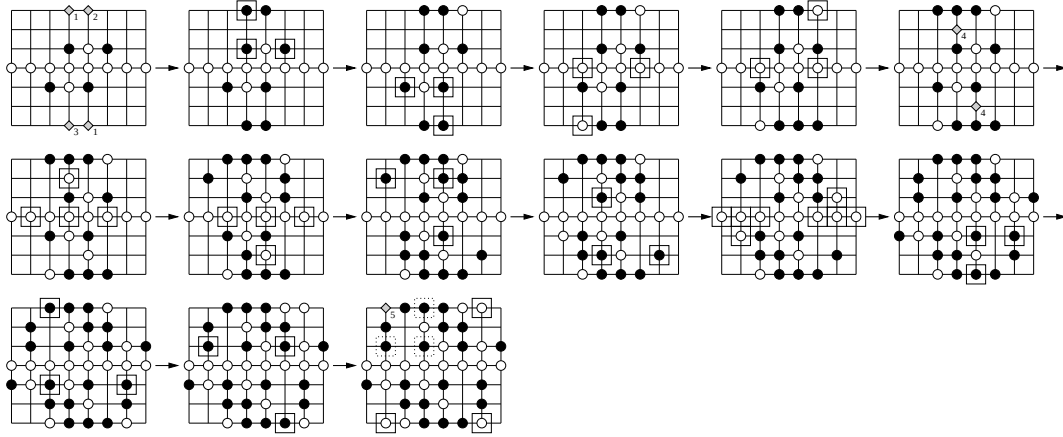
FIGURE 13. Under the hypothesis that the diamonds marked 1, 2, and 3 all have color \bullet , the diamonds marked 4 must have color \circ (stacked rows). The diamond marked 5 cannot be colored.
