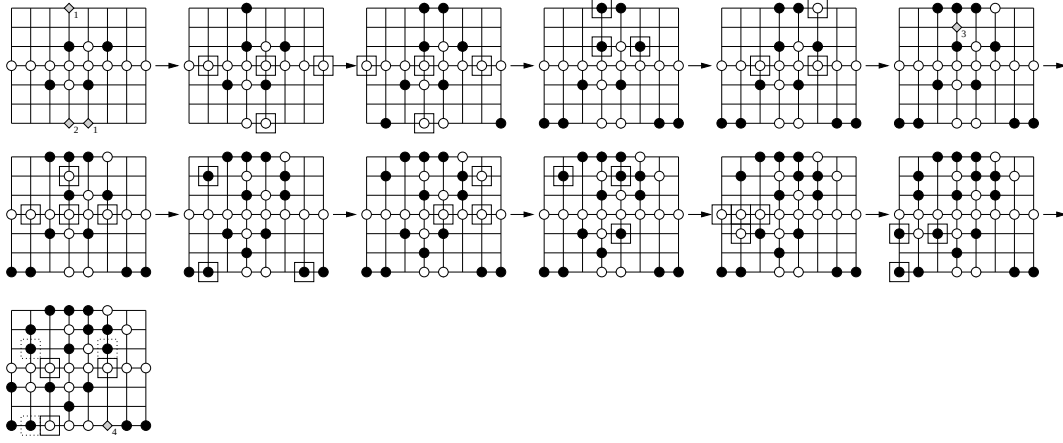
FIGURE 17. Under the hypothesis that one of the diamonds marked 1 has color \circ and the other has color \bullet and that the diamond marked 2 has color \circ , the diamond marked 3 must have color \circ (stacked rows). The diamond marked 4 cannot be colored. This concludes the proof of case 4.
