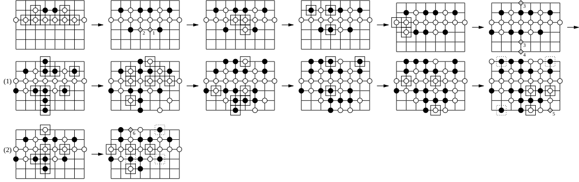
FIGURE 9. The diamonds marked 1 and 2 cannot both have color \circ . Without loss of generality (due to symmetry), we color the diamond marked 1 \circ . Since the diamonds marked 3 cannot both have color \circ , we examine the cases where both have color \bullet and where one has color \bullet and the other has color \circ . Similarly, either the diamond marked 4 or the vertex above the upper diamond marked 3 must have color \bullet , so by symmetry we say that the diamond marked 4 has color \bullet . (1) examines the case where both diamonds marked 3 have color \bullet ; here, the diamond marked 5 cannot be colored. (2) examines the case where one diamond marked 3 has color \circ and the other has color \bullet ; here, the diamond marked 6 cannot be colored. This concludes the proof of case 3.
