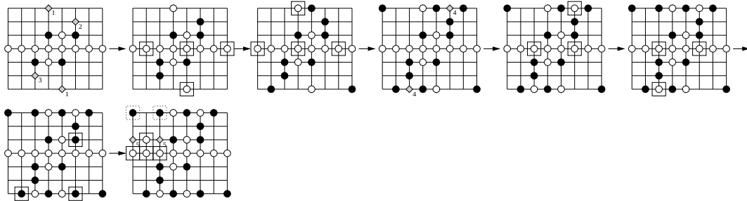
FIGURE 11. Under the hypothesis that the diamonds marked 1 have color \circ , and the diamonds marked 2 and 3 have color \bullet , the diamond marked 4 must have color \circ (staggered rows). The diamonds marked 5 cannot be colored.
