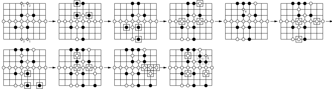
FIGURE 14. Under the hypothesis that both diamonds marked 1 have color \bullet , the diamond marked 2 has color \bullet , and the diamond marked 3 has color \circ , the diamond marked 4 must have color \circ (stacked rows). This shows that the diamond marked 5 cannot be colored. (We need not consider the case where the diamond marked 2 has color \circ and the diamond marked 3 has color \bullet ; we use symmetry to take care of this.)
